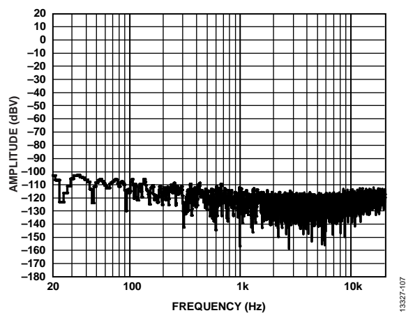
Figure 13. FFT, No Signal, Analog Gain = 14, R_L = 4\ \Omega
