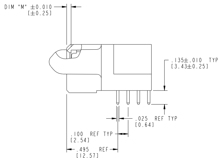
BROKEN-OUT SECTION B-B SCALE 2:1
