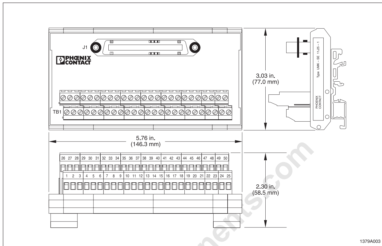
Figure 2. TELCO Dimensions
