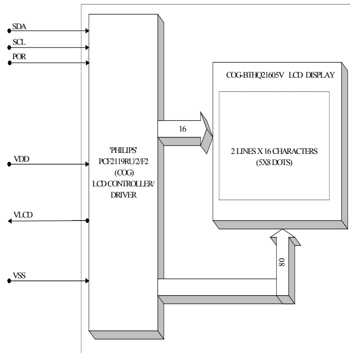
Figure 4: Block Diagram
