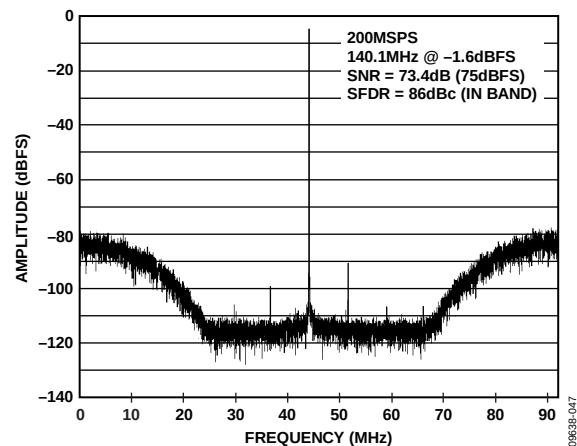
Figure 54. 22% BW Mode, Tuning Word = 28 ( f_s/4 Tuning)
