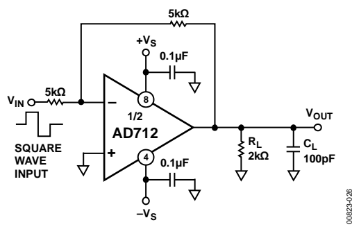
Figure 26. Unity-Gain Inverter
