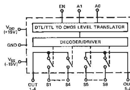
AD7502
