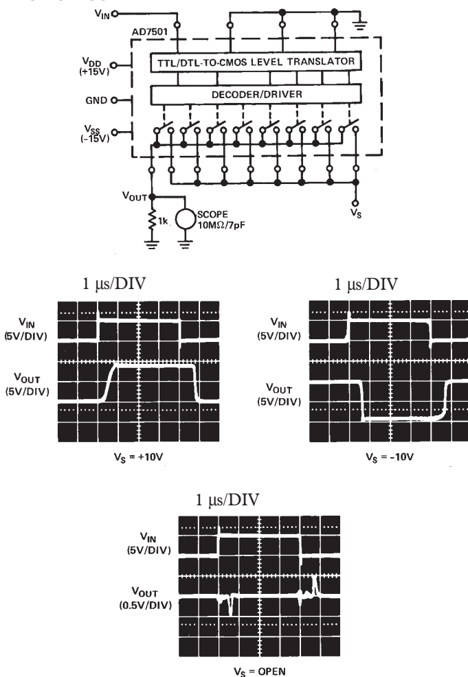
TEST CIRCUIT 2
