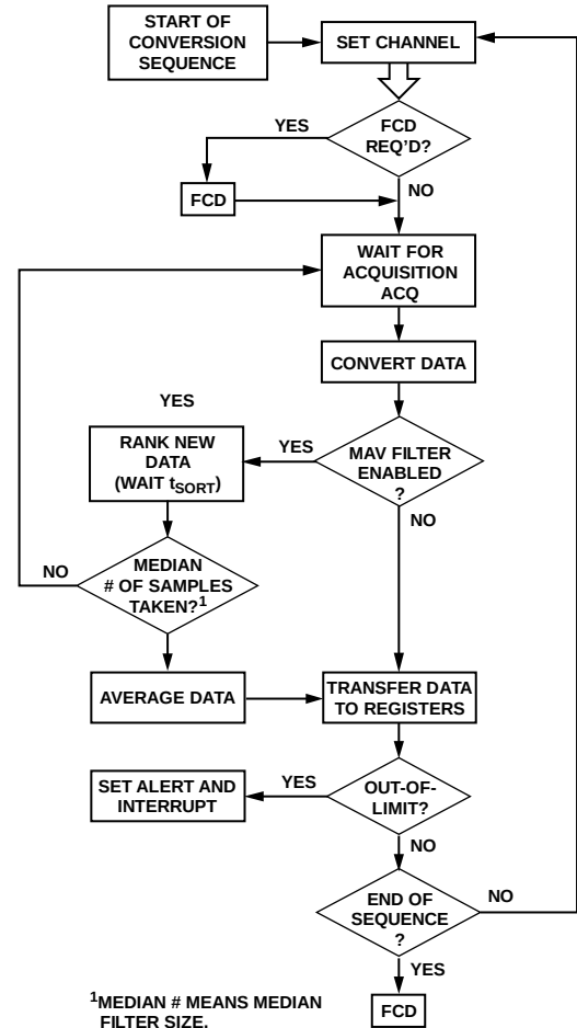
Figure 34. Conversion Sequence
