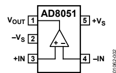
Figure 2. SOT-23-5 (RJ)
