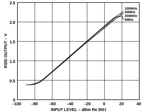
Figure 31. RSSI Output vs. Input Level at T_A = +25^\circ\text{C} , for Frequencies of 5 MHz, 50 MHz, 100 MHz and 200 MHz
