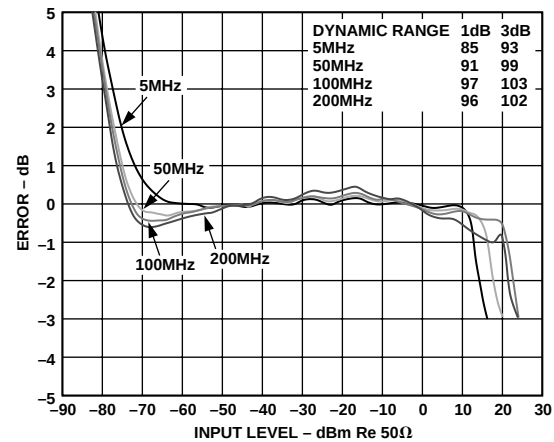
Figure 32. Log Linearity vs. Input Level at T_A = +25^\circ\text{C} , for Frequencies of 5 MHz, 50 MHz, 100 MHz and 200 MHz
