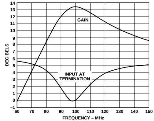
Figure 34. Response of 100 MHz Matching Network
