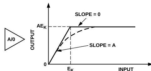
Figure 23. A/0 Amplifier Functions (Ideal and tanh)
