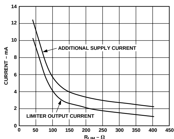
Figure 17. Additional Supply Current and Limiter Output Current vs. R_{\text{LIM}}
