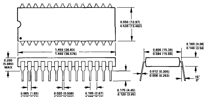
28-Pin Plastic DIP Package
