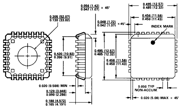
28-Pin PLCC Package
