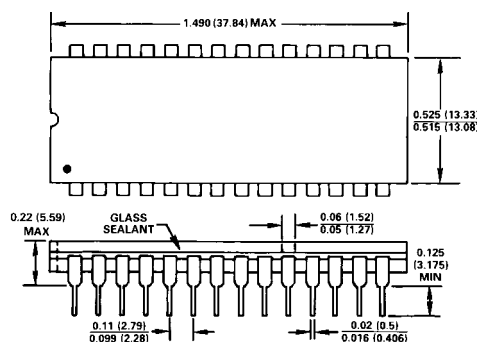
28-Pin Cerdip
