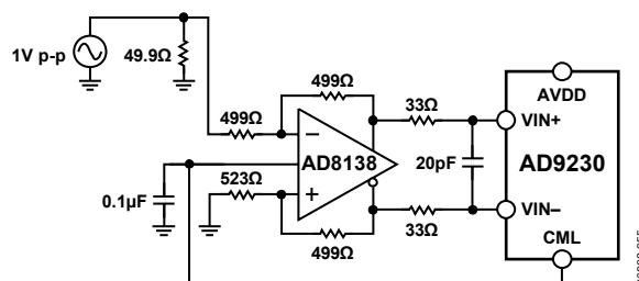
Figure 52. Differential Input Configuration Using the AD8138
