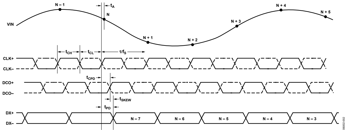
Figure 2. Single Data Rate Mode
