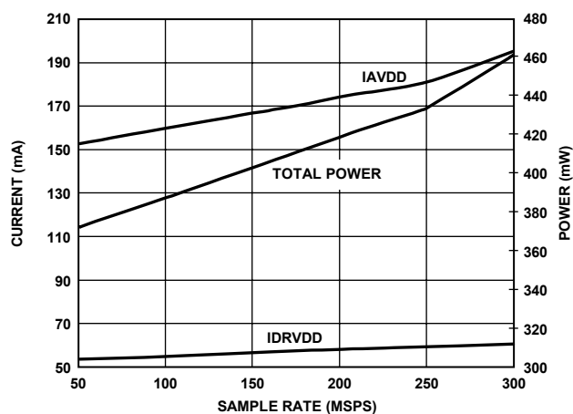
Figure 42. AD9230 Power Supply Current vs. Sample Rate
