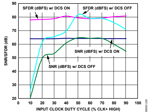
Figure 49. SNR/SFDR vs. Sample Clock Duty Cycle; 250 MSPS, 170.3 MHz @ -1 dBFS
