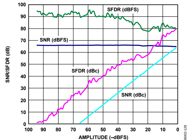
Figure 39. AD9230-250 SNR/SFDR vs. Input Amplitude; 250 MSPS, 170.3 MHz
