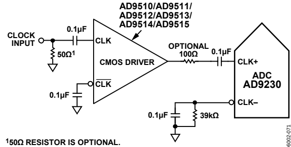
Figure 58. Single-Ended 1.8 V CMOS Sample Clock
