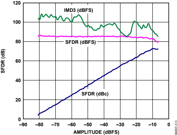
Figure 22. AD9230-170 Two-Tone SFDR vs. Input Amplitude; 170 MSPS, 140.1 MHz, 141.1 MHz
