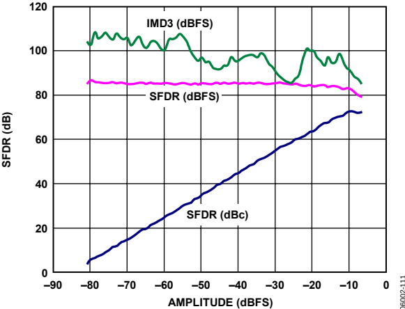
Figure 33. AD9230-210 Two-Tone SFDR vs. Input Amplitude; 210 MSPS, 170.1 MHz, 171.1 MHz
