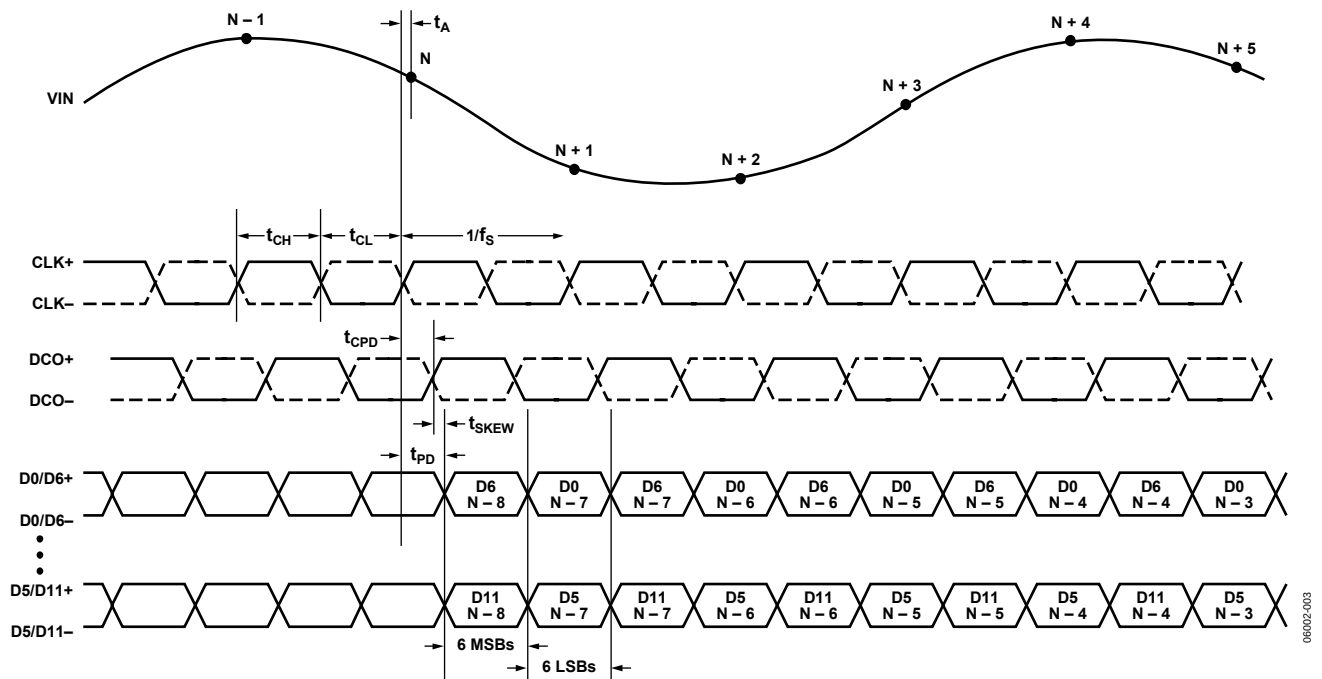
Figure 3. Double Data Rate Mode
