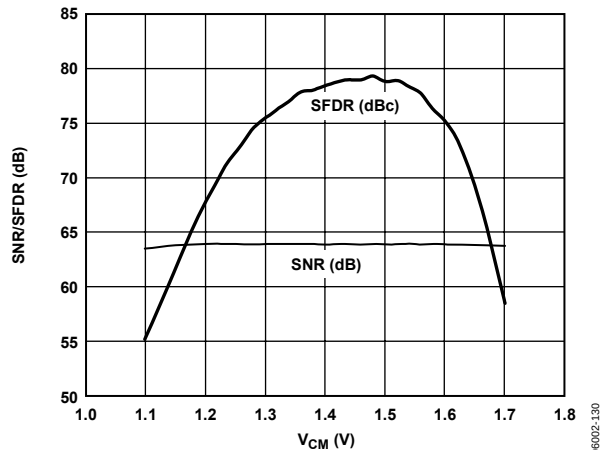
Figure 46. SNR/SFDR vs. Common-Mode Voltage; 250 MSPS, 70.3 MHz @ -1 dBFS
