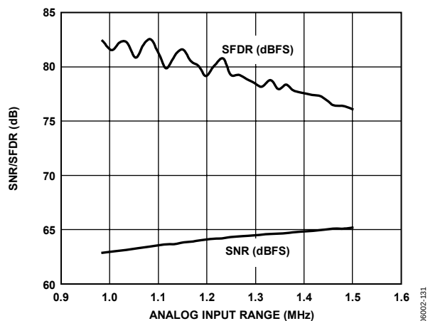
Figure 48. SNR/SFDR vs. Analog Input Range; 250 MSPS, 170.3 MHz @ -1 dBFS
