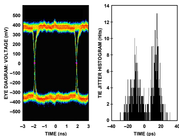
Figure 61. Data Eye for LVDS Outputs in ANSI Mode with Trace Lengths Less than 24 Inches on Standard FR-4, AD9230-250
