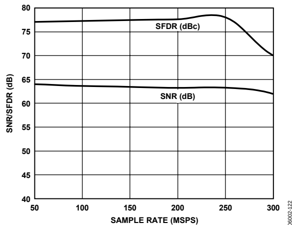
Figure 47. SNR/SFDR vs. Sample Rate; 250 MSPS, 170.3 MHz @ -1 dBFS
