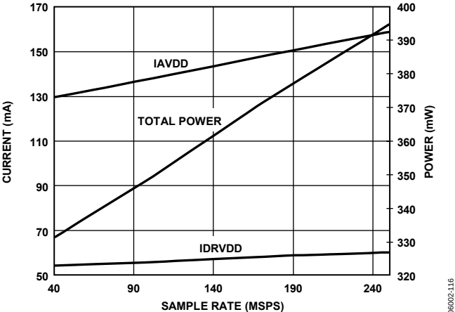
Figure 31. AD9230-210 Power Supply Current vs. Sample Rate
