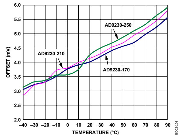
Figure 51. Offset vs. Temperature
