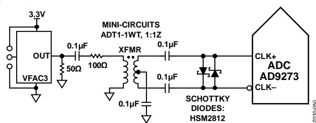
Figure 55. Transformer-Coupled Differential Clock
