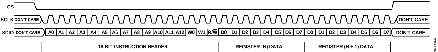
Figure 68. Serial Control Port Write—LSB First, 16-Bit Instruction, Two Bytes Data
