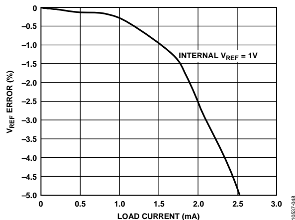
Figure 53. V_{REF} Error vs. Load Current
