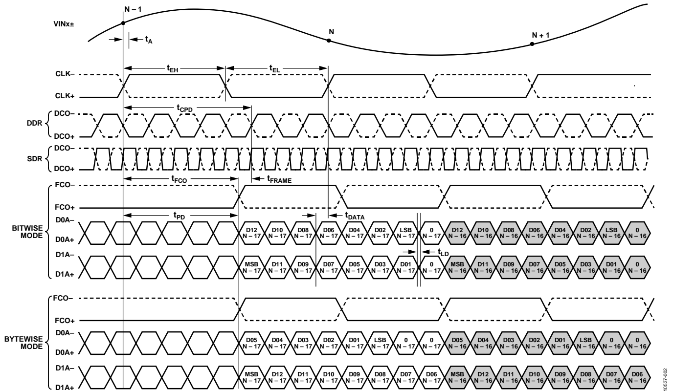
Figure 2. 16-Bit DDR/SDR, Two-Lane, 1x Frame Mode (Default)
