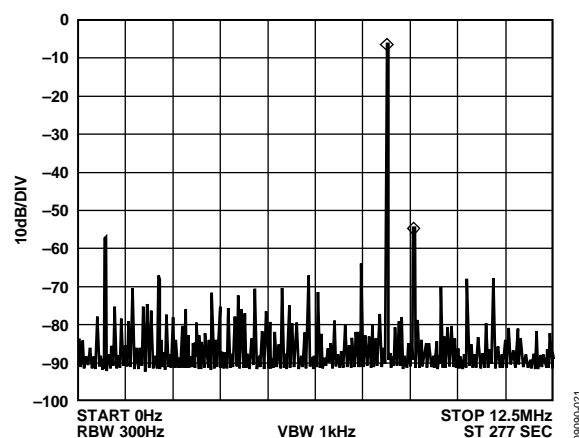
Figure 21. f_{MCLK} = 25 MHz, f_{OUT} = 8.1 MHz, Frequency Word = 0x52F1A9FC
