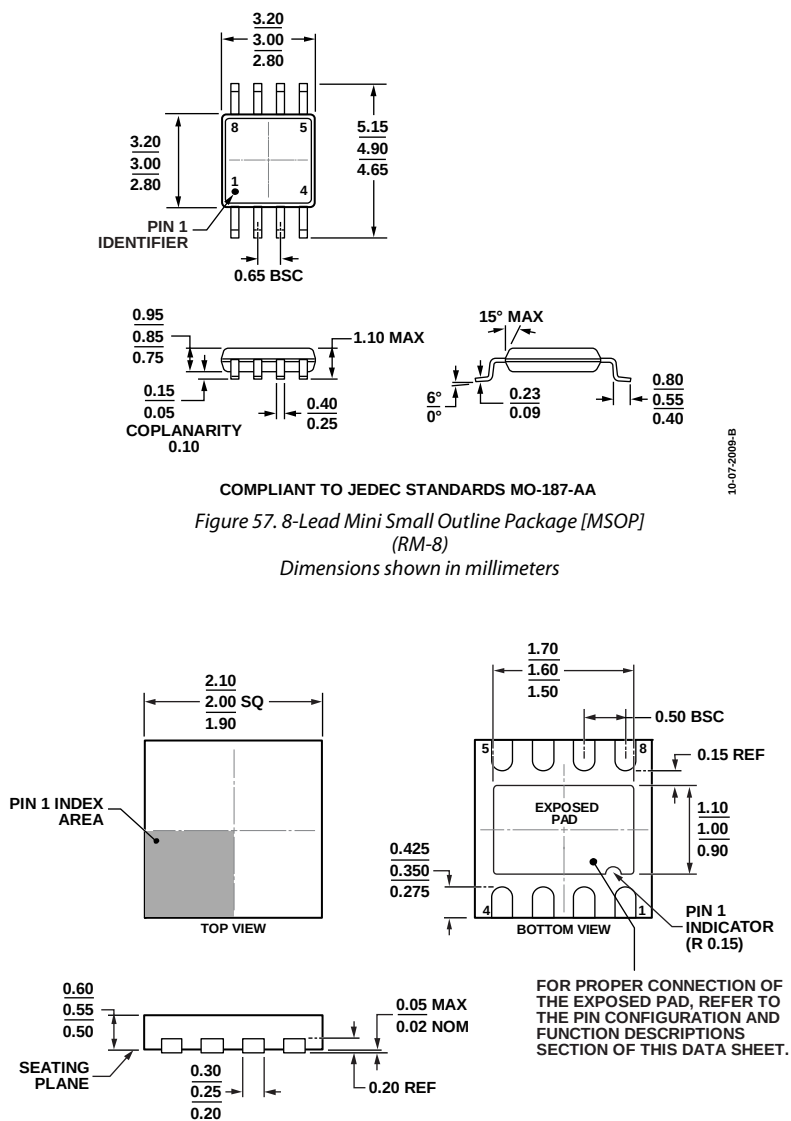
Figure 58. 8-Lead Lead Frame Chip Scale Package [LFCSP_UD] 2 mm x 2 mm Body, Ultra Thin, Dual Lead (CP-8-10) Dimensions shown in millimeters
