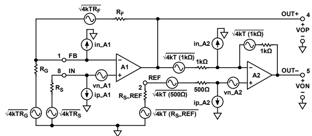
Figure 53. Noise Sources
