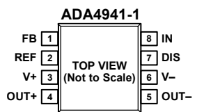
Figure 5. 8-Lead SOIC Pin Configuration
