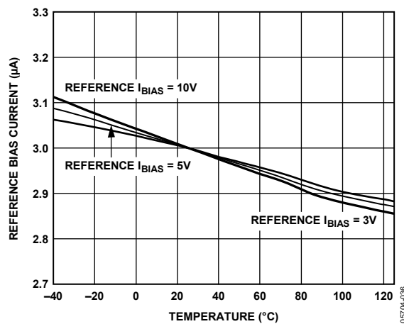
Figure 38. REF Input Bias Current vs. Temperature
