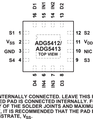
Figure 3. LFCSP Pin Configuration
