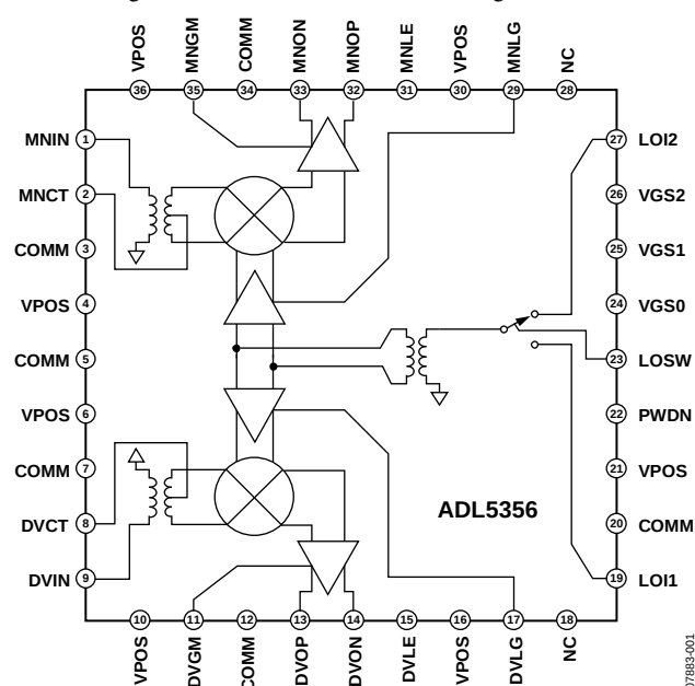
Figure 52. Simplified Schematic
