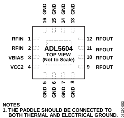
Figure 3. Pin Configuration
