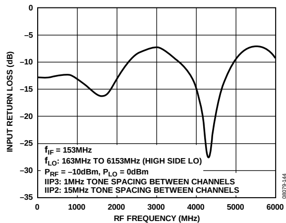
Figure 109. Input Return Loss vs. RF Frequency
