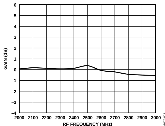
Figure 27. Power Conversion Gain vs. RF Frequency
