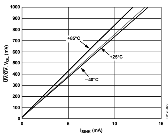
Figure 14. \overline{UV}/\overline{OL} Voltage Output Low vs. Output Sink Current
