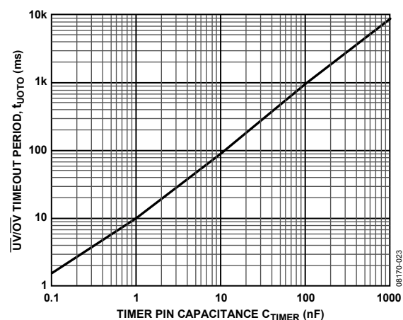
Figure 15. \overline{UV}/\overline{OL} Timeout Period vs. Capacitance
