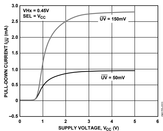
Figure 13. I_{SINK} , I_{OL} vs. V_{CC}
