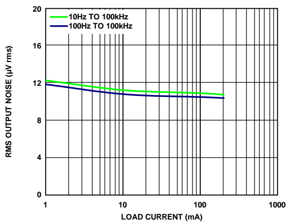
Figure 32. RMS Output Noise vs. Load Current ( I_{LOAD} )
