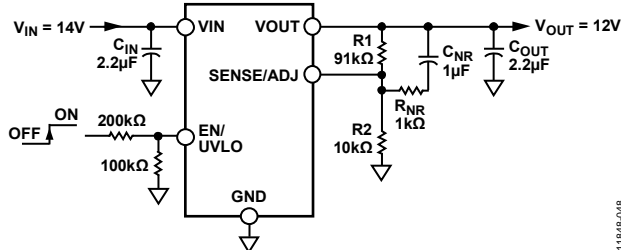
Figure 50. Noise Reduction Modification
