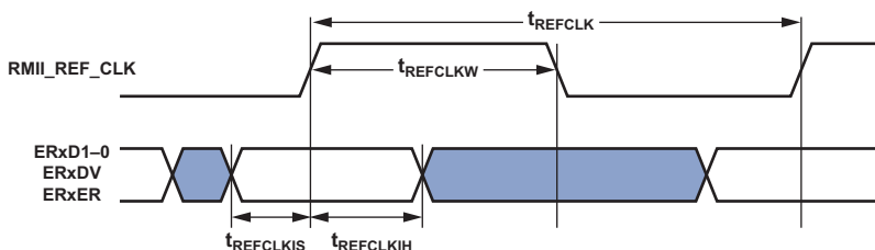
Figure 38. 10/100 Ethernet MAC Controller Timing: RMII Receive Signal
