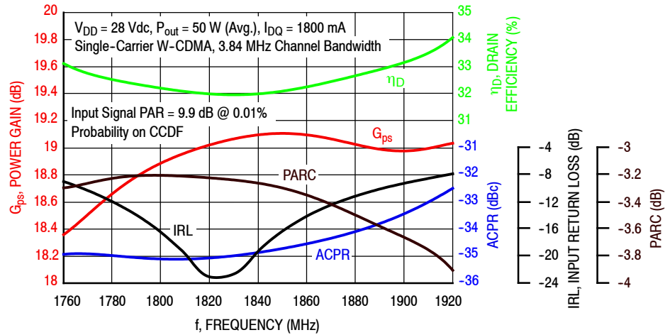
Figure 3. Single-Carrier Output Peak-to-Average Ratio Compression (PARC) Broadband Performance @ P_{out} = 50 \text{ Watts Avg.}
