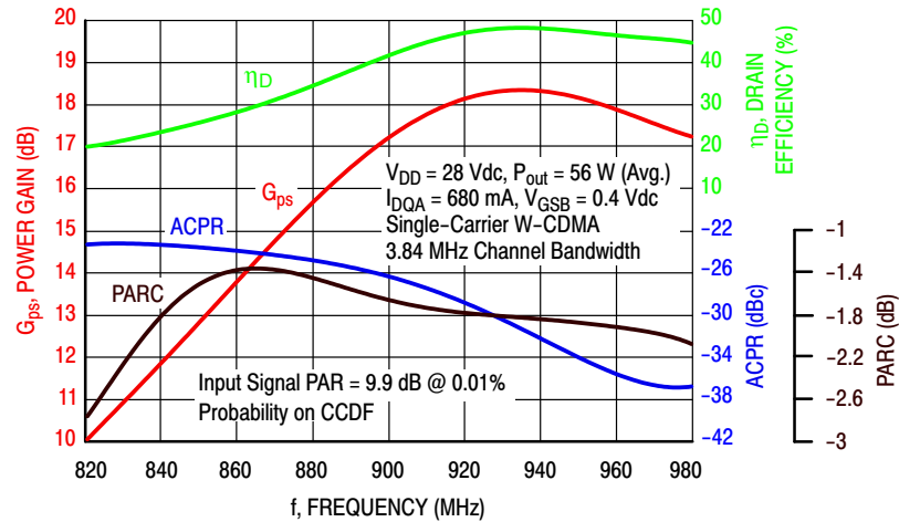
Figure 3. Single-Carrier Output Peak-to-Average Ratio Compression (PARC) Broadband Performance @ P_{out} = 56 \text{ Watts Avg.}
