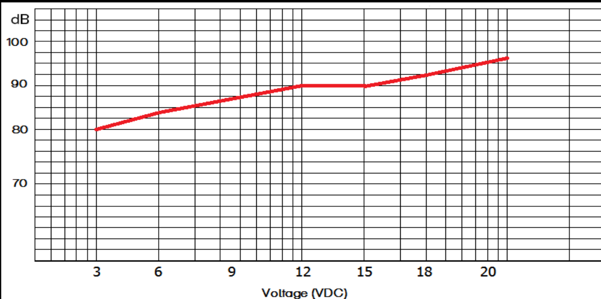
SPL vs Voltage (measured @ 10 cm)
