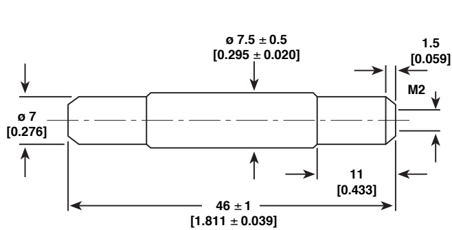
Figure 1: GWK 10
