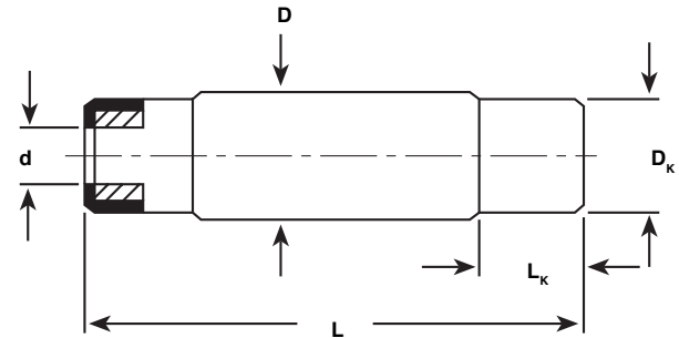
Figure 2: GWK 20...GWK 300
