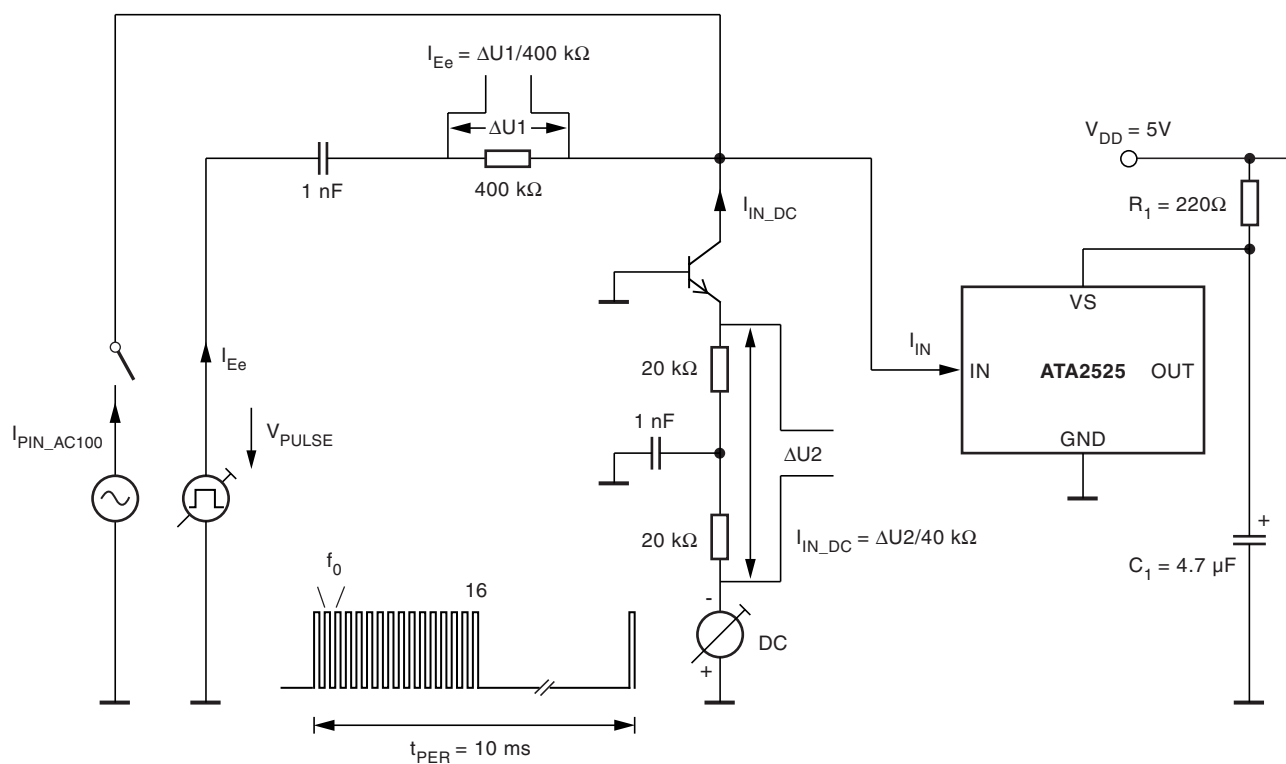
Figure 6-6. Test Circuit
