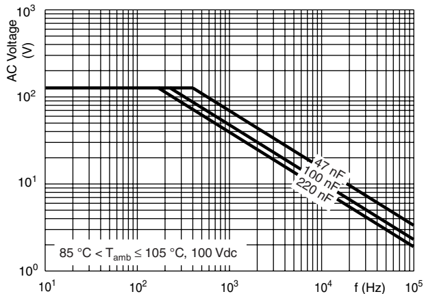
377 - Max. AC voltage as a function of frequency
