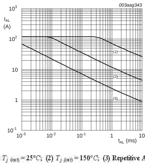
Fig 3. Single-pulse and repetitive avalanche rating; avalanche current as a function of avalanche time
