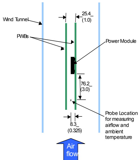
Figure 34. Thermal Test Set-up.
