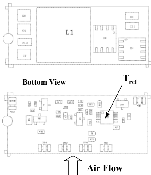
Figure 33. T ref Temperature measurement location.
