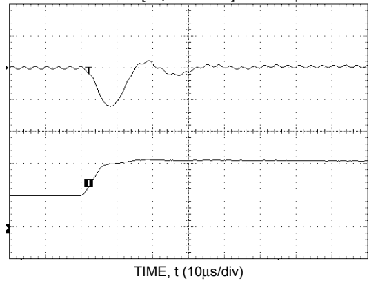
Figure 10. Transient Response to Dynamic Load Change from 50% to 100% of full load ( V_O = 3.3Vdc ).
