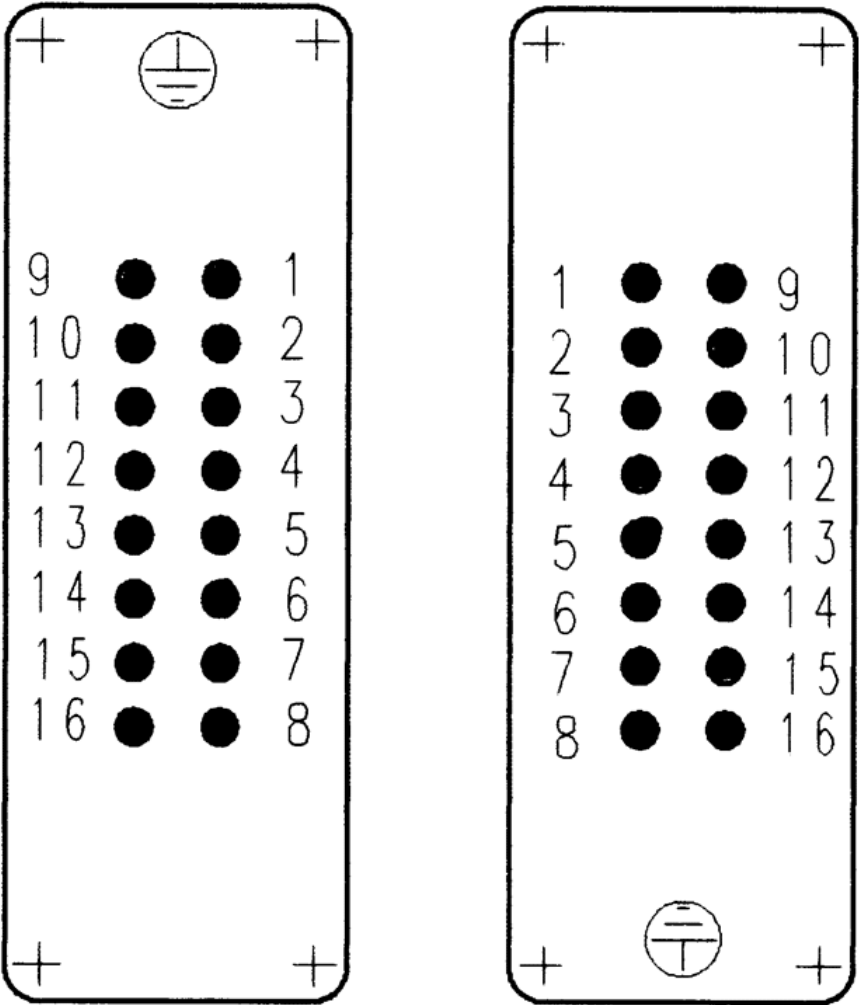
Contact arrangement
