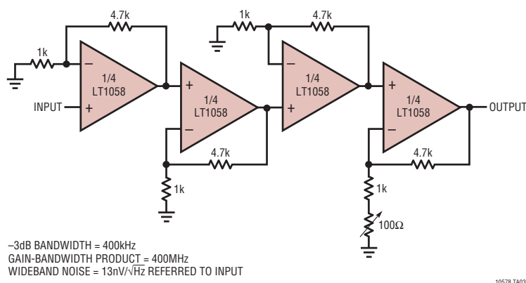
Wideband, High Input Impedance, Gain = 1000 Amplifier
