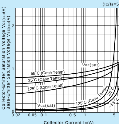
VCE(sat), VBE(sat)-IC Temperature Characteristics (Typical)
