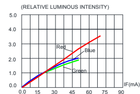
FIG.2 RELATIVE LUMINOUS INTENSITY VS. FORWARD CURRENT
