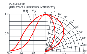
FIG.6b RED FAR FIELD PATTERN
