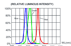
FIG.5 RELATIVE LUMINOUS INTENSITY VS. WAVELENGTH.
