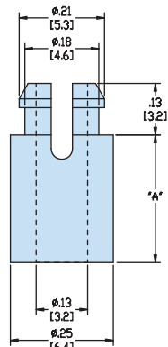
TWO PRONG SNAP LOCK / #4 or M3 SELF-TAPPING SCREW
