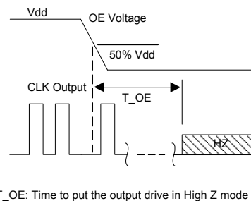
Figure 6. OE Disable Timing (OE Mode Only)
