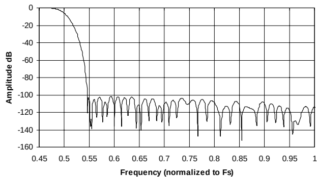
Figure 8. Operational Mode 0 Stopband Rejection
