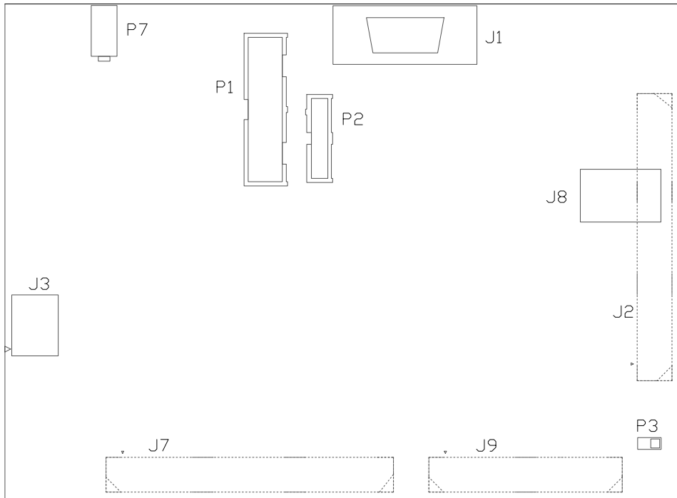
Figure 2-9. Connector Locations
