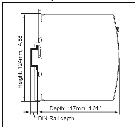
Fig. 22-2 Side view
