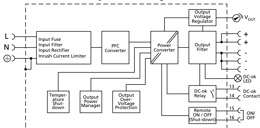
Fig. 12-1 Functional diagram
