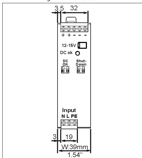
Fig. 22-1 Front view
