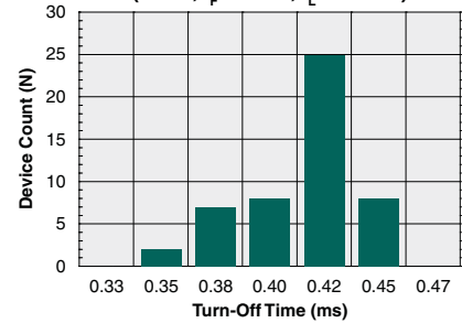
Typical Turn-Off Time (N=50, I_F=10\text{mA} , I_L=140\text{mA} )
