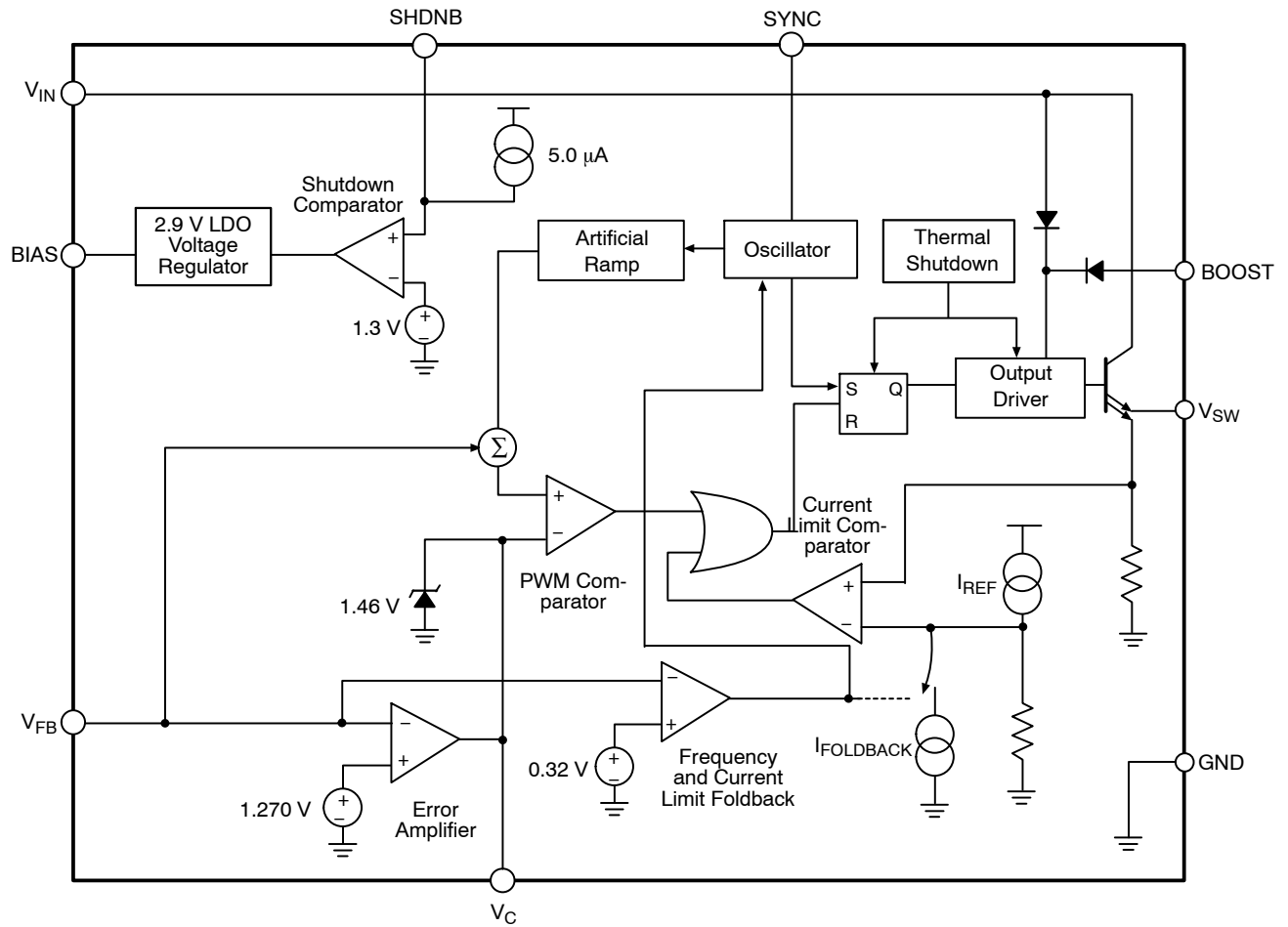
Figure 2. Block Diagram
