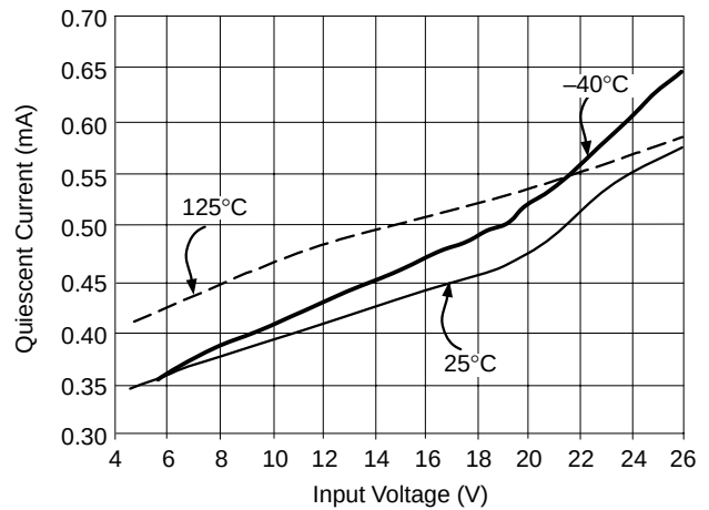
Figure 7. Quiescent Current vs. Input Voltage I_{OUT} = 100\text{ }\mu\text{A}
