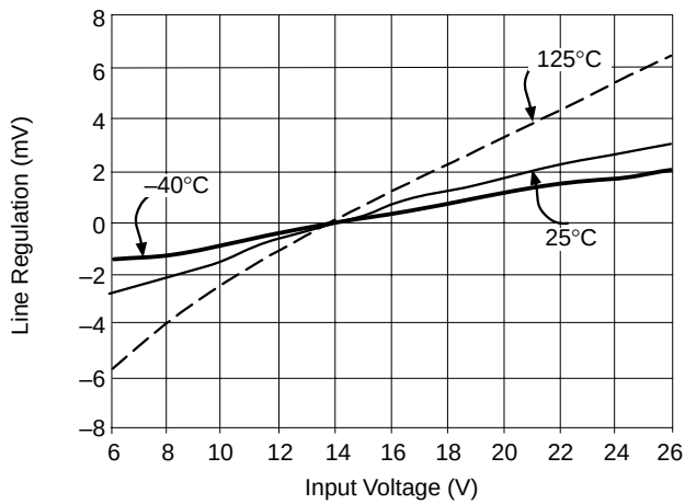
Figure 4. Line Regulation vs. Input Voltage I_{OUT} = 100\text{ }\mu\text{A}
