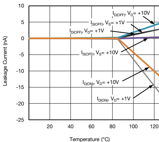
Leakage Current vs. Temperature ( +12\text{ V} )
