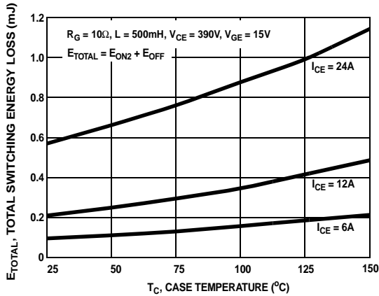
Figure 15. Total Switching Energy Loss vs Case Temperature
