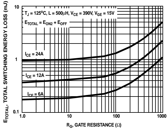
Figure 16. Total Switching Energy Loss vs Gate Resistance
