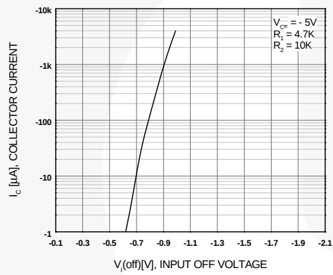
Figure 3. Input-Off Voltage
