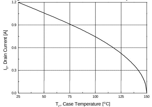
Fig 10. Max. Drain Current vs. Case Temperature
