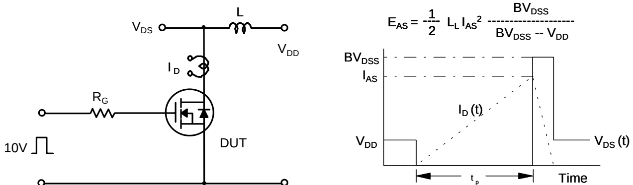
Fig 14. Unclamped Inductive Switching Test Circuit &amp; Waveforms
