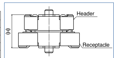
(H):Reference dimension
